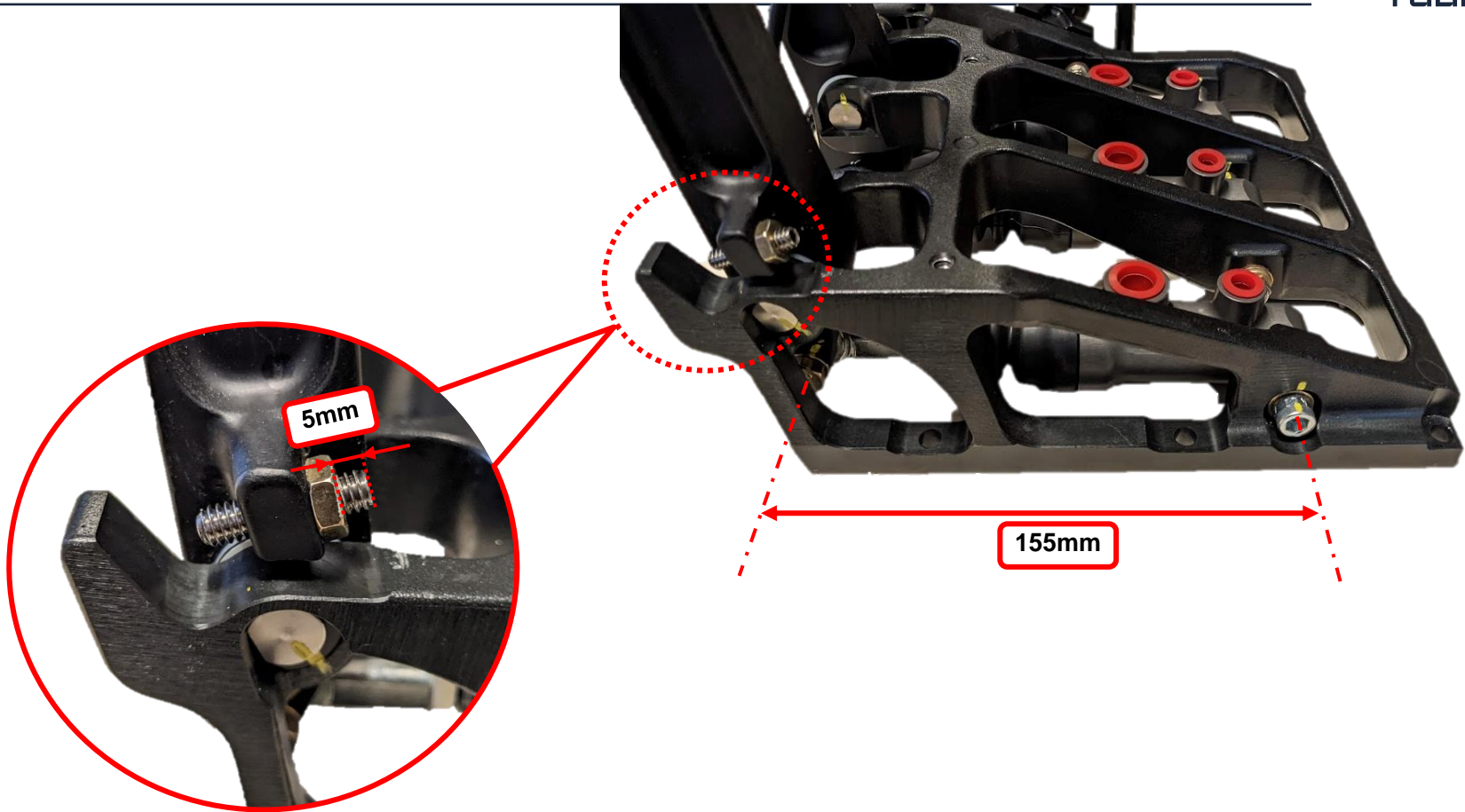
Clutch pedal setup
