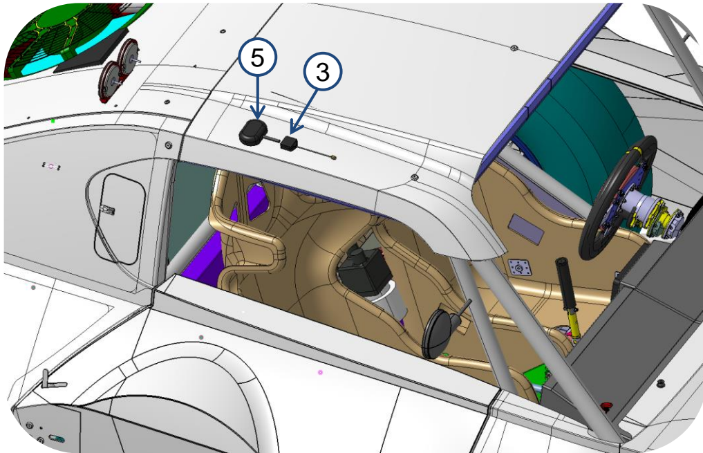
Position antennas according to drilling templates
