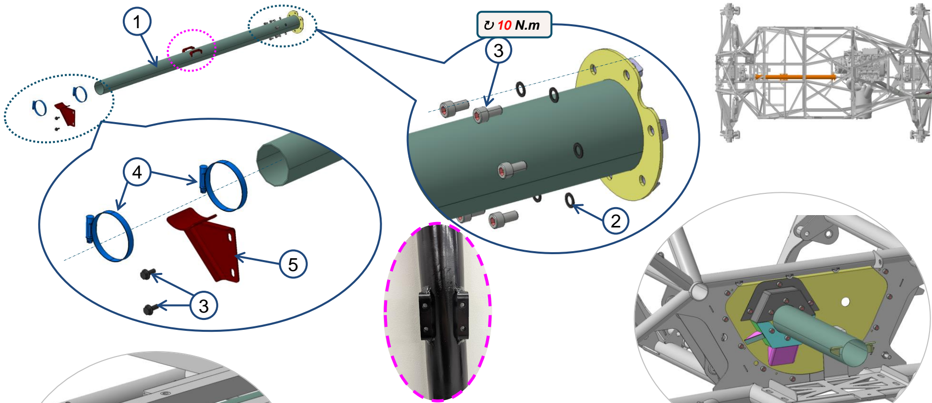
Bracket for machined gear lever
